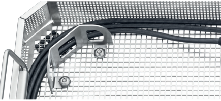
GB072R ECCOS® >> GA805/806
